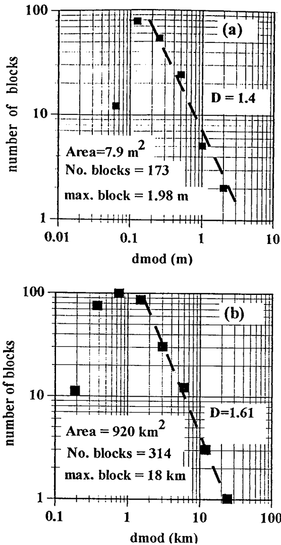
Figure 4 Log-histograms of block sizes from two disparate sources and measurement areas (m 2 and km 2 ): a) shows data from the same outcrop as image in Figure 3; b) shows data from source geology maps used in the preparation of Figure 2; (both from Medley, 1994a).
