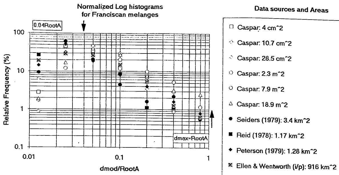
Figure 5 Compilation of log-histograms for Franciscan melanges. RootA is \sqrt{A} .
